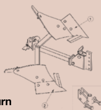
1 Plough 1/4 turn - detail
