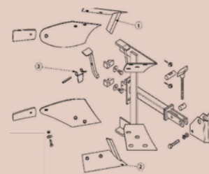
2 Plough 1/2 turn - detail
