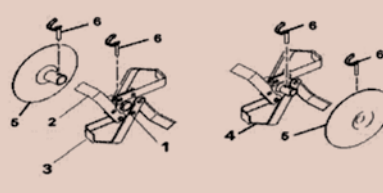
7 - Farming tool 119: 06726-733-003HE Hexagonal shaft 23 mm
